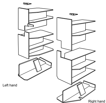
Multi Pass 90/110 Baffle System
