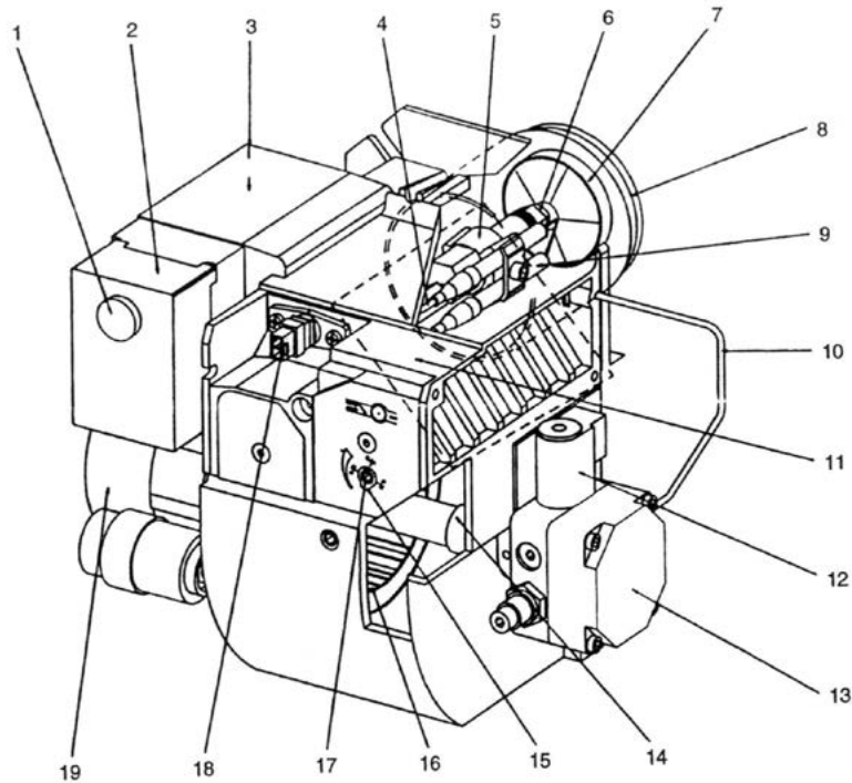
Sterling Burner [Exploded View]
