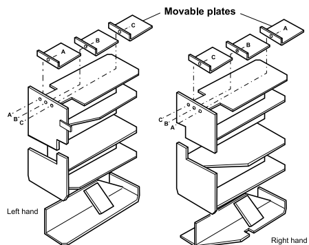
Multi Pass 70/90 Baffle System
