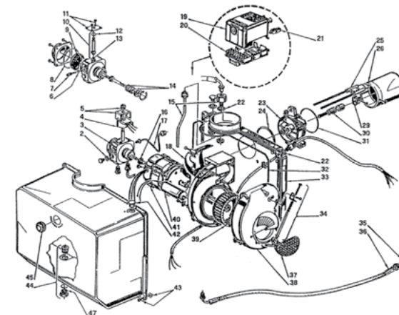
Riello G5 Burner [Exploded View]
