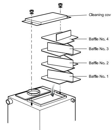
Euroflame 50/70 & Combi 70 Baffle System
