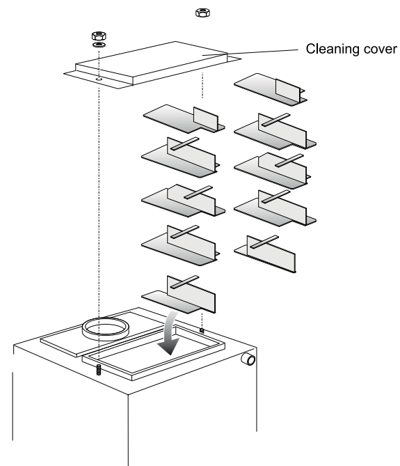
Euroflame 90/120 Baffle System
