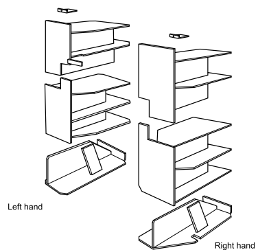
Multi Pass 160/200 Baffle System
