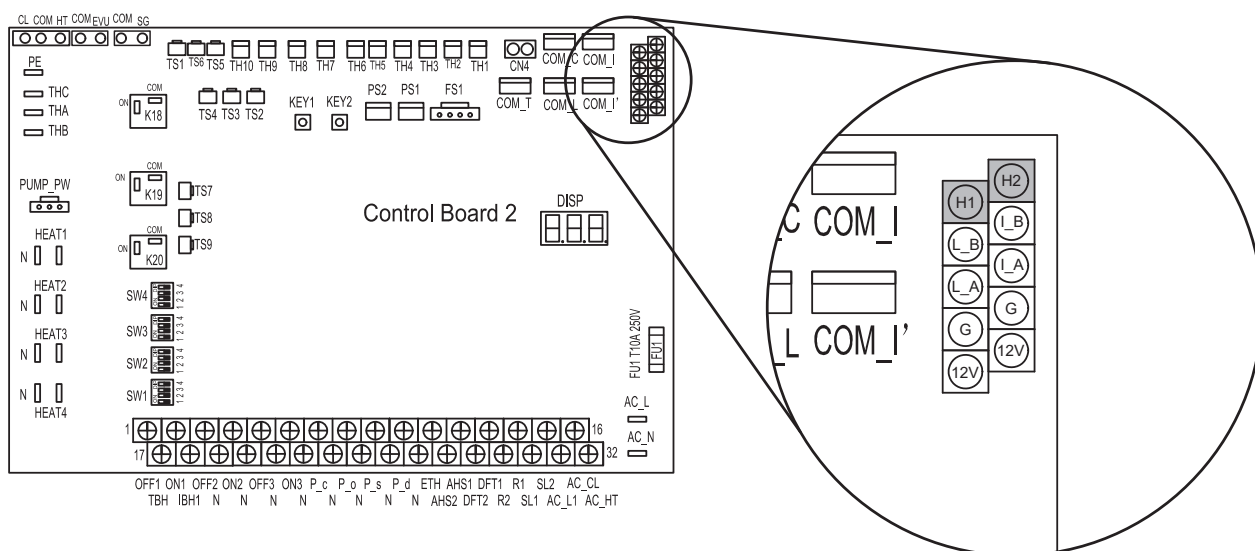
Figure 3-9: Modbus connection to Grant Aeron R290 Heat pump
