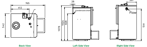
Vortex Boiler House 46-70kW
