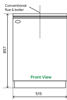
Vortex Pro Combi XS 26kW
