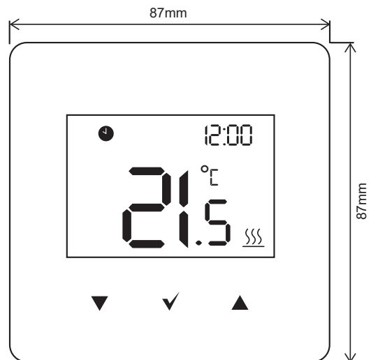
Figure A-4: Wired (& Wireless) thermostat panel LCD
