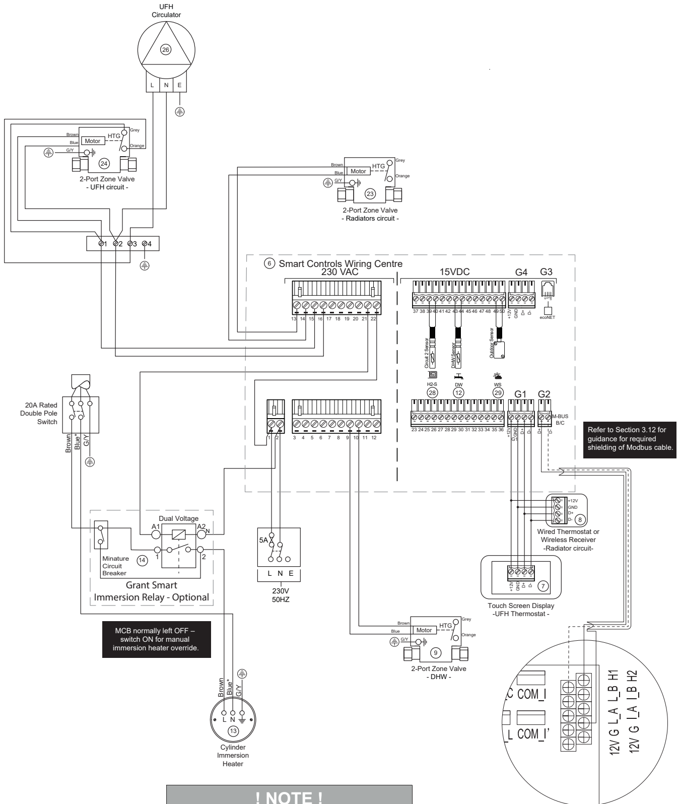
① Grant Aeron 290 Hydraulic PCB
