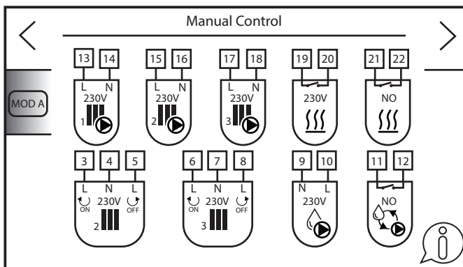
Figure 8-2: Manual Control
