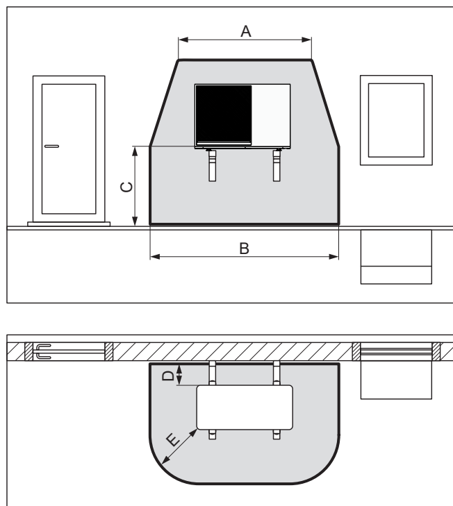
Figure 3-9: Wall installation in a low position
