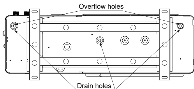
Figure 3-15: Drain and overflow holes - 4 kW
