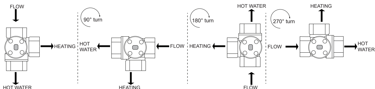
Figure B-1: Valve positions
