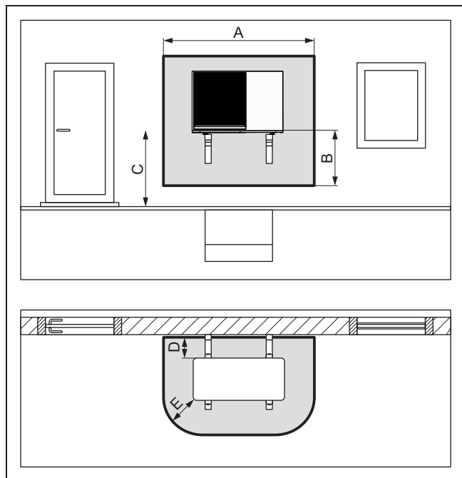
Figure 3-10: Raised wall installation
