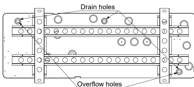
Figure 3-17: Drain and overflow holes - 12 kW & 15.5 kW
