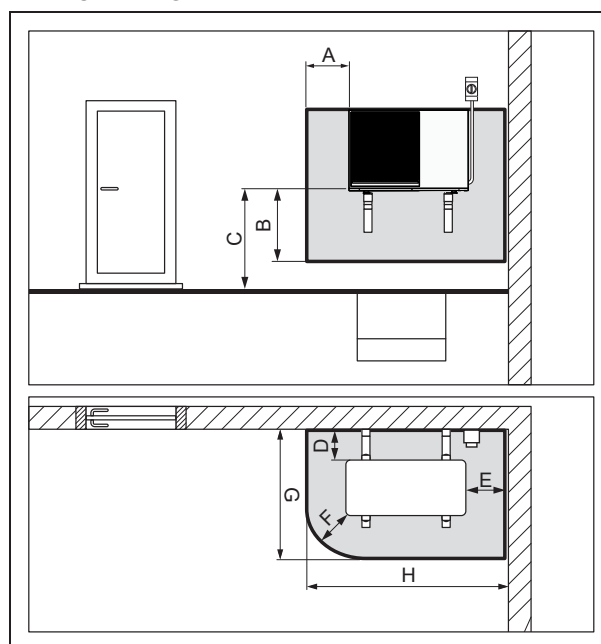
Figure 3-12: Right corner wall installation above opening
