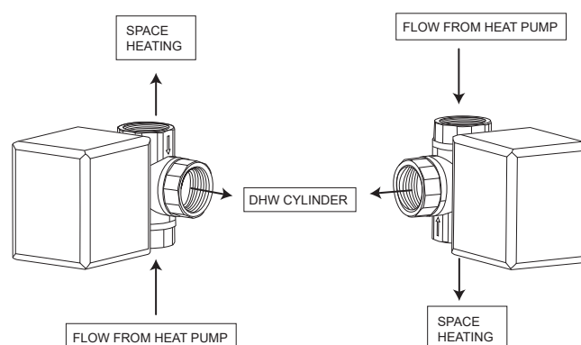
Figure B-2: Valve Position 1
