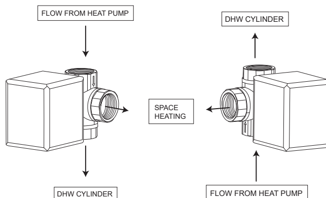
Figure B-3: Valve Position 2
