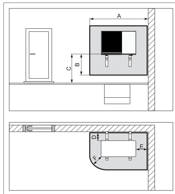
Figure 3-12: Raised Wall installation in a right-hand corner
