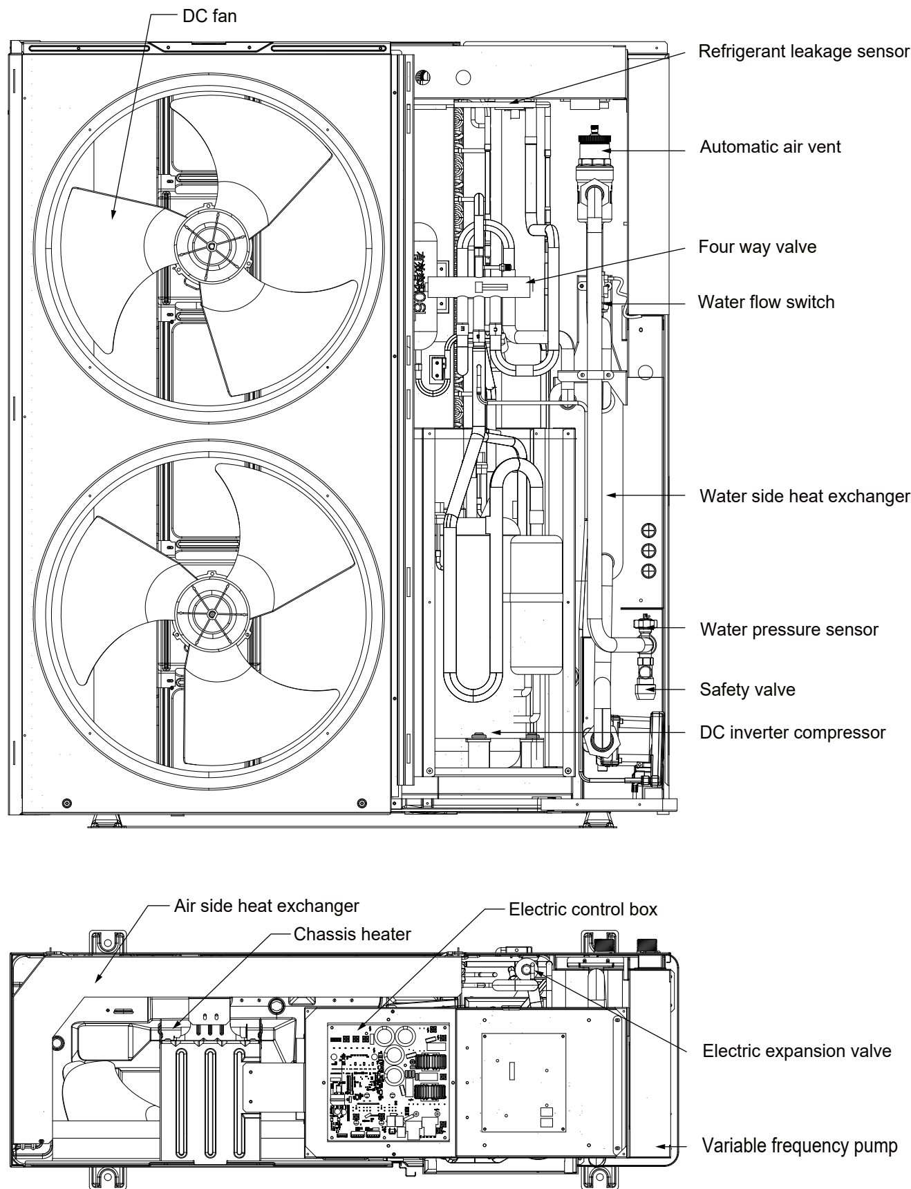
Figure 1-4: Main components - HPR290155
