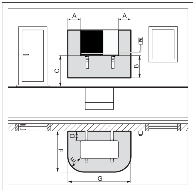
Figure 3-10: Wall installation above opening
