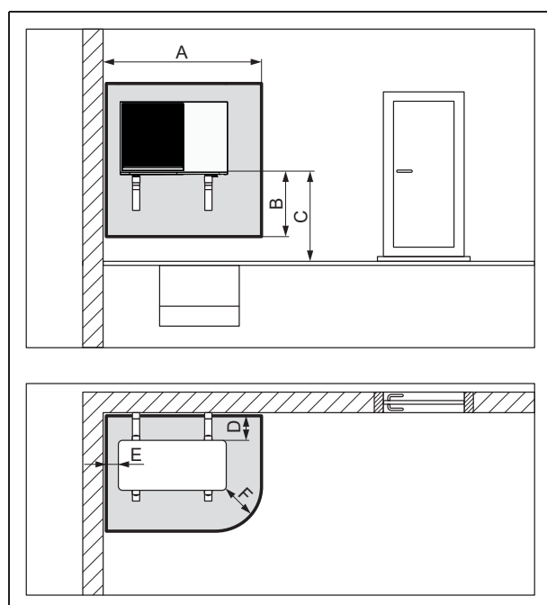
Figure 3-11: Raised Wall installation in a left-hand corner
