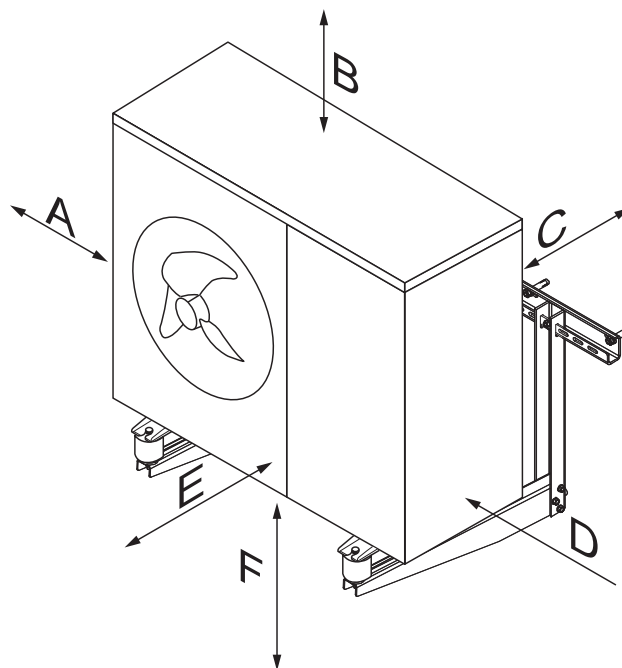
Figure 3-14: Wall mounted installation clearances
