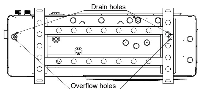
Figure 3-16: Drain and overflow holes - 6.5 kW & 9 kW
