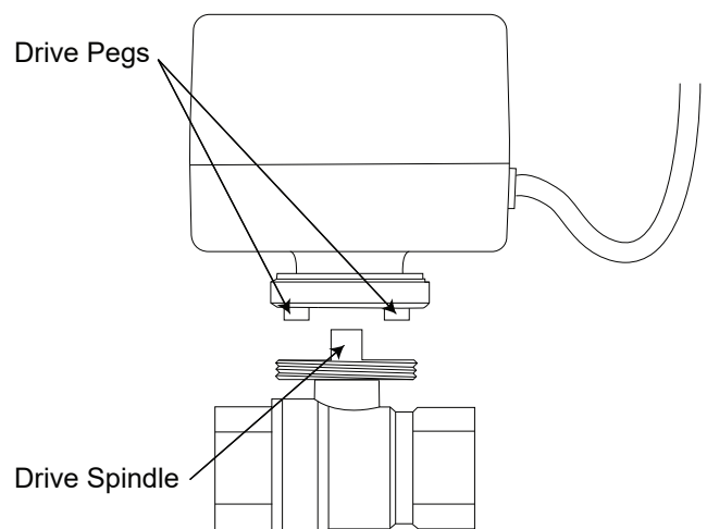
Figure B-7: Drive pegs and drive spindle
