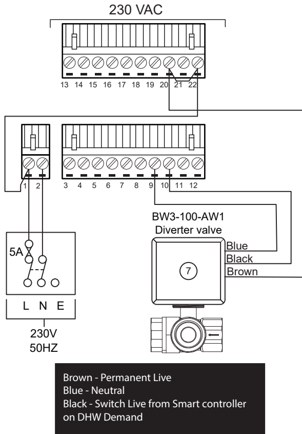
Figure B-8: Smart Controller wiring
