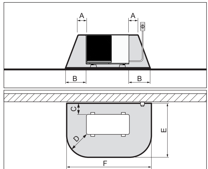
Figure 3-7: Ground installation in front of a building
