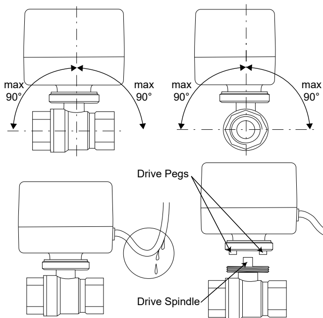
Figure B-1: Actuator & Valve
