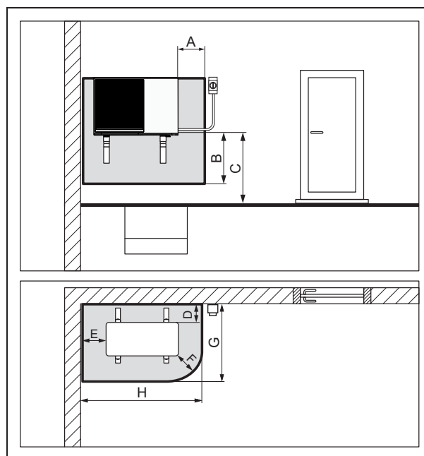
Figure 3-11: Left corner wall installation above opening
