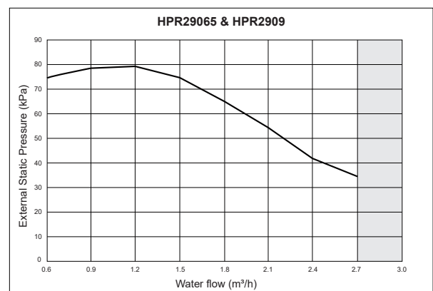
Figure 8-8: Pressure Loss Performance HPR29065 & HPR29065
