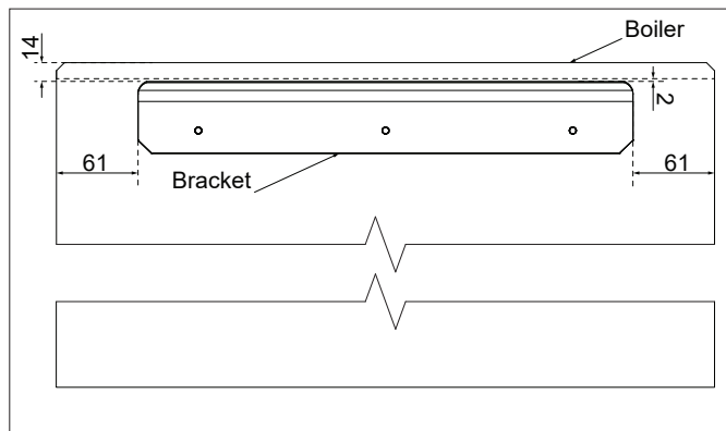
Figure 3-1: Upper and side dimensions between the EvoLink and the bracket
