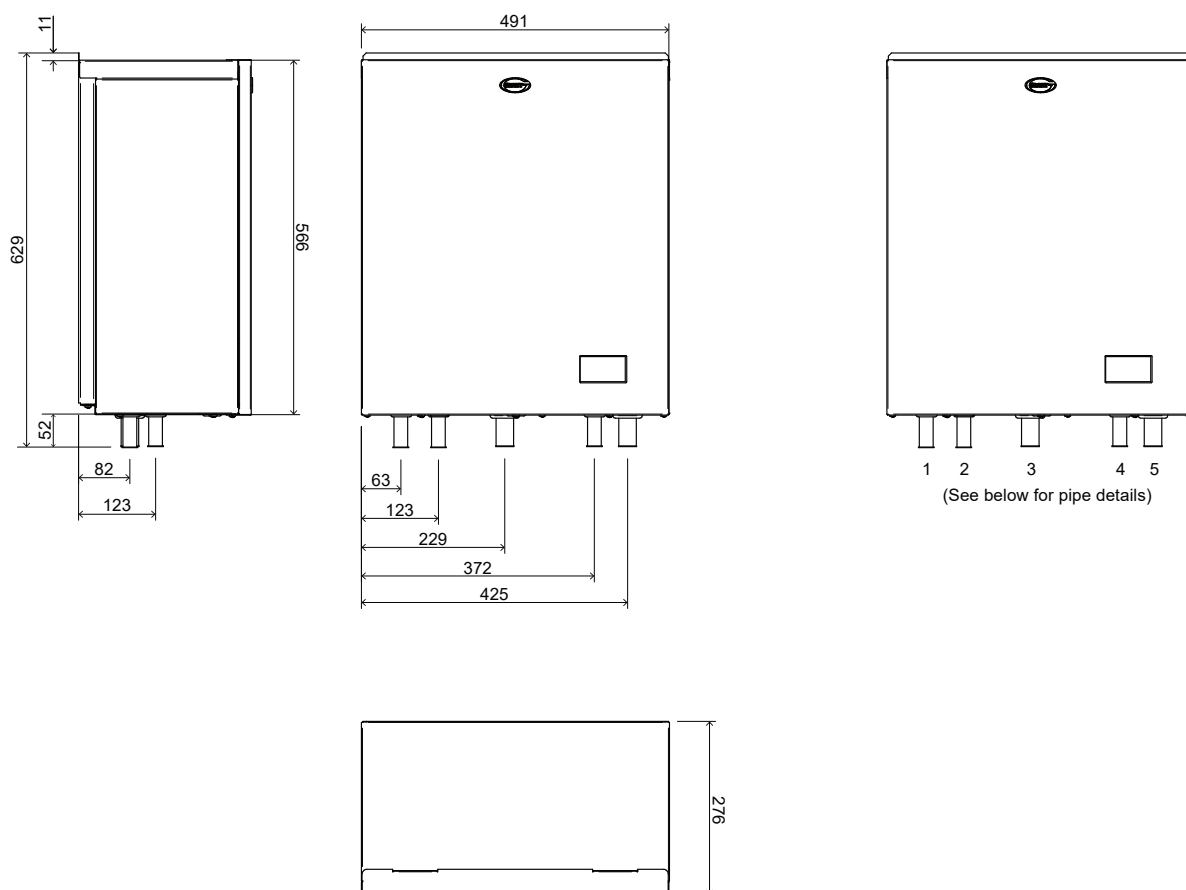
Figure 2-1: EvoLink Dimensions
