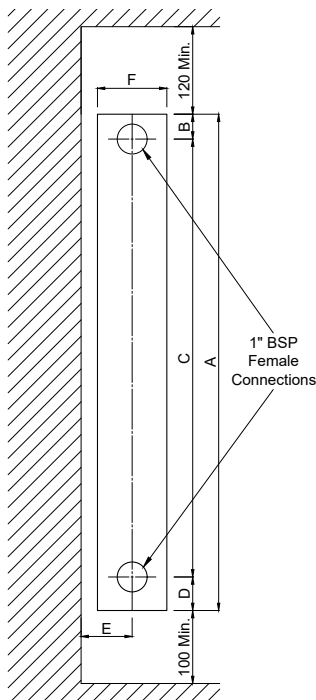
Figure 3-1: Radiator Clearances and Dimensions Section 3: Installation
