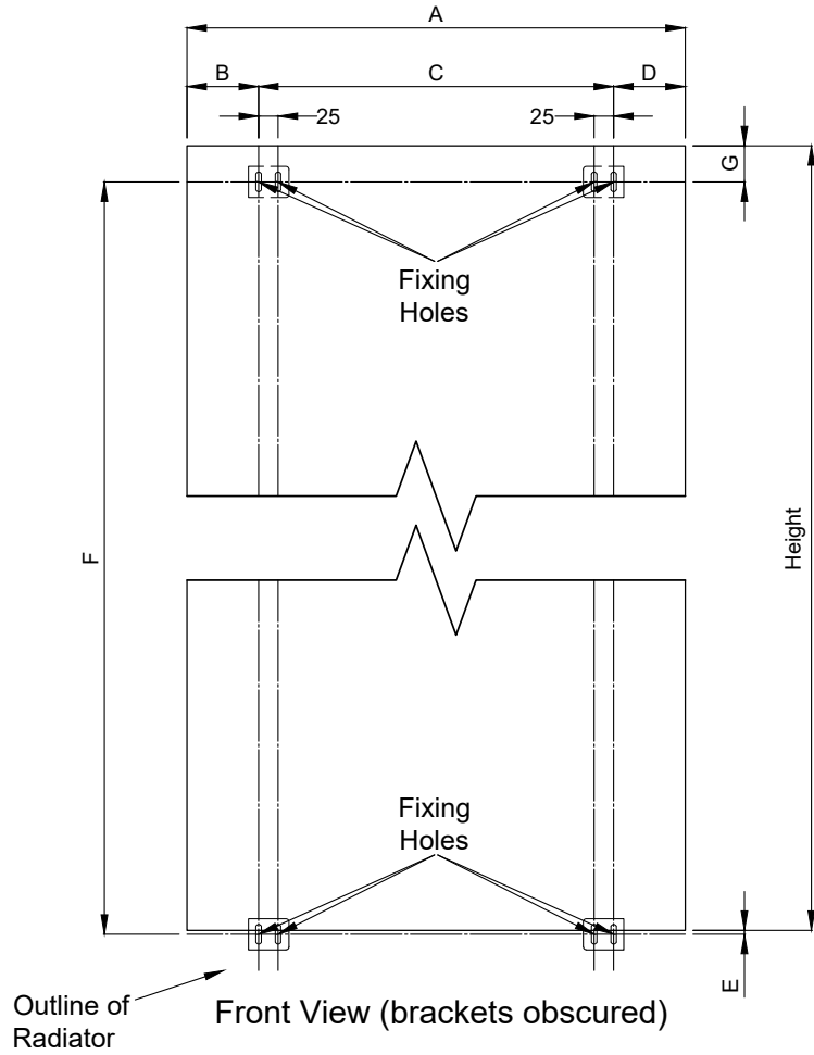
Figure 3-7: Fixing hole positions for Vertical radiators
