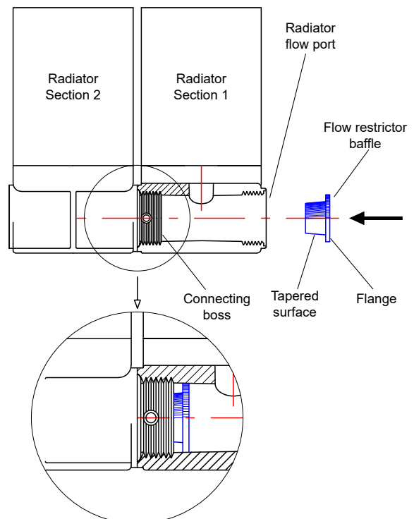
Figure 3-2: Fitting flow restrictor baffle
