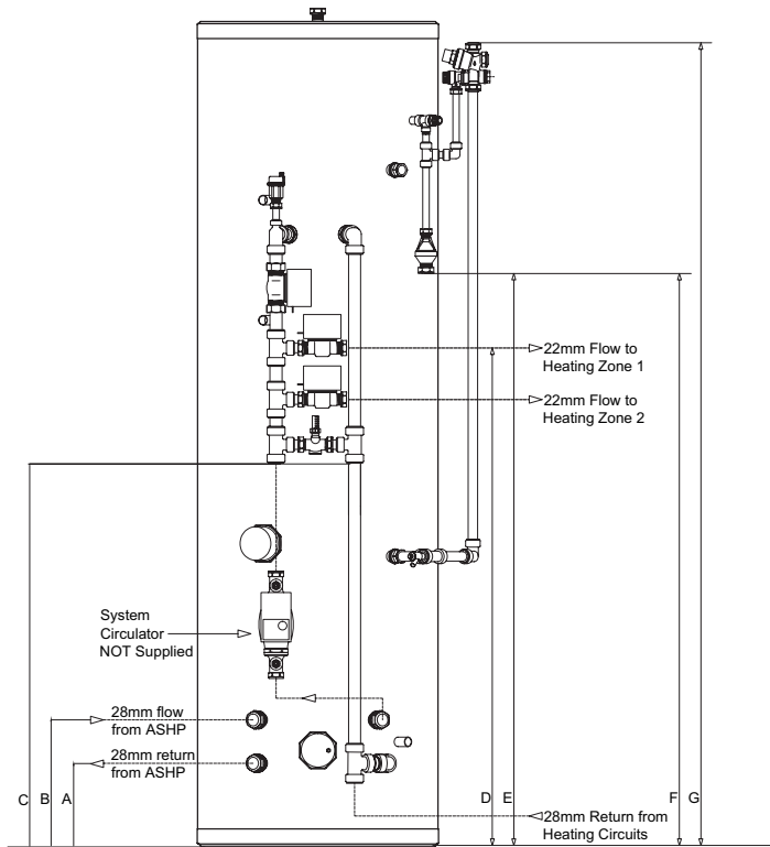
Pre-plumbed cylinder (buffer option)
