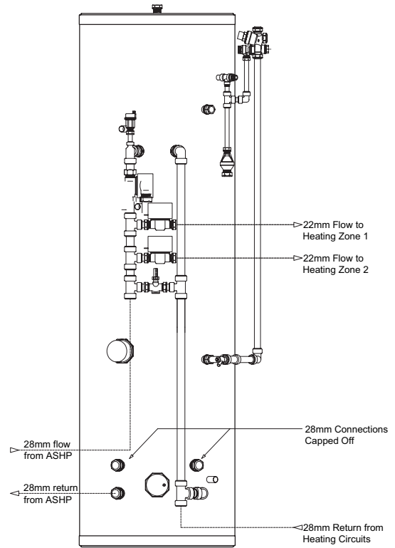
Pre-plumbed cylinder (volumiser option)
